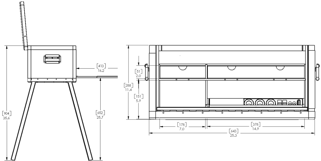
side view and front view [mm] inch
